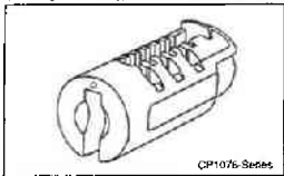
PLUG-SUB ASSEMBLY (Retaining Tumblers Only)
